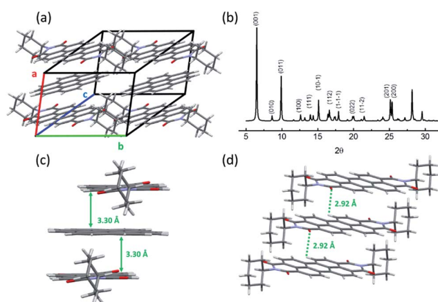
Fig. 2 (a) Triclinic cell showing the alternate stacking of coronene and PTCDI in the cocrystal. (b) XRD spectrum recorded on the cocrystal. (c) The \pi – \pi stacking between coronene and PTCDI-C6 with a spacing of 3.30 Å. (d) The hydrogen bonds between the perylene hydrogen and the imide oxygen of nearby PTCDIs.
