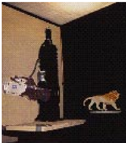
Figure 9: Our prototype camera gantry. A modified Cyberware MS motion platform with additional stepping motors from Lin-Tech and Parker provide four degrees of freedom: horizontal and vertical translation, pan, and tilt. The camera is a Panasonic WV-F300 3-CCD video camera with a Canon f/1.7 10-120mm zoom lens. We keep it locked off at its widest setting (10mm) and mounted so that the pitch and yaw axes pass through the center of projection. While digitizing, the camera is kept pointed at the center of the focal plane. Calibrations and alignments are verified with the aid of a Faro digitizing arm, which is accurate to 0.3 mm.
