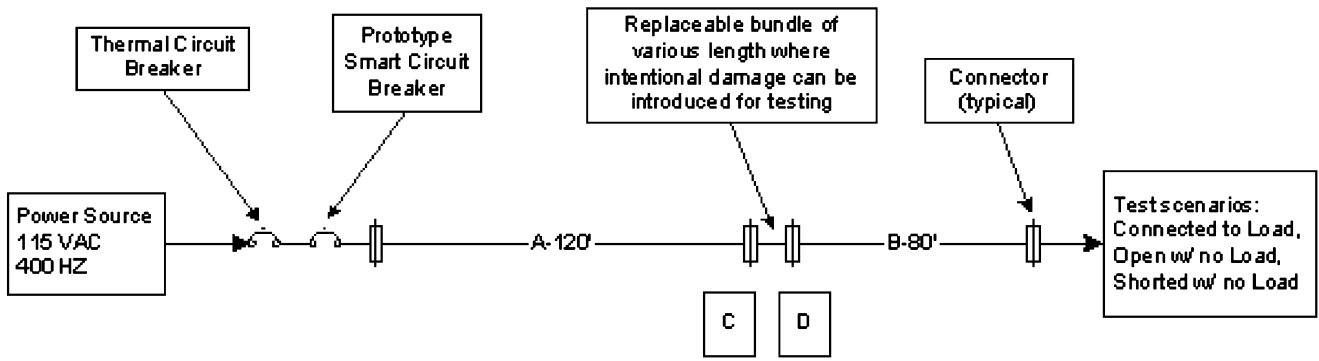
Fig. 3. Boeing wiring test bench.
