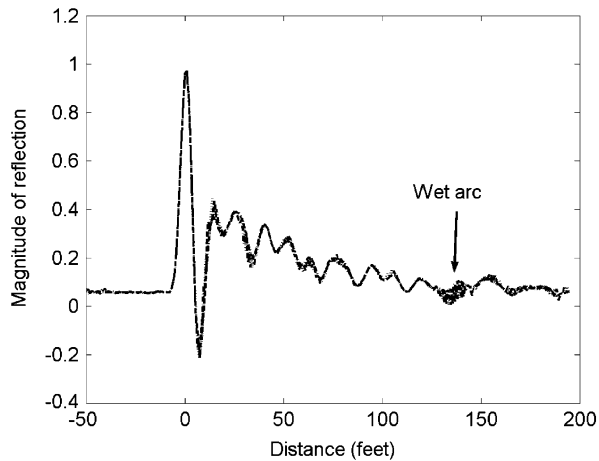
Fig. 7. STDR traces showing the instantaneous near short circuits caused when saline solution is dripped on a wire with damaged insulation, making a partial path for conduction. Several time samples are superimposed to show the location of the wet arc.
