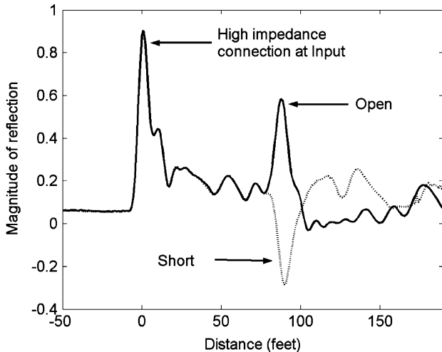
Fig. 2. STDR response for an 80-ft wire (paired single 22 gauge wires bundled with other wires) that is short or open circuited on the end.
