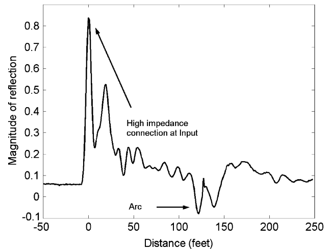
Fig. 6. STDR traces showing the instantaneous near short circuits caused when saline solution is dripped on a wire with damaged insulation, making a partial path for conduction.
