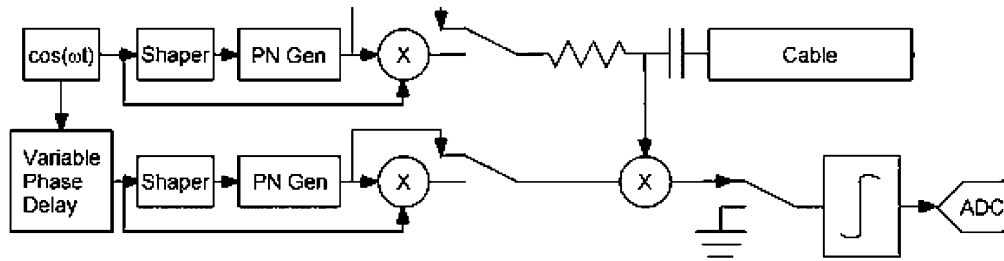
Fig. 1. Circuit diagram for STDR/SSTDR system.
