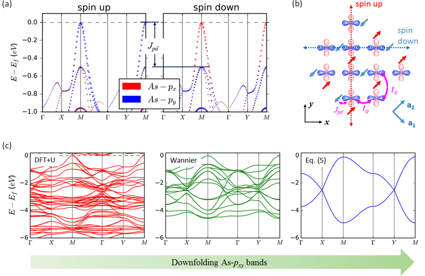
FIG. 5. Hoppings and spin polarization of the As - p_{xy} orbitals and formation of the hole bands in NaFe_{0.5}Cu_{0.5}As . (a) Spin- and orbital-resolved valence bands. The bands are projected on the p_{xy} orbitals of a single As atom. The p_y/p_x bands around the Fermi level are found to carry the opposite spin. The splitting between the spin-up and spin-down pockets of the same orbital is used to estimate J_{pd} . (b) Schematics of the p - p hopping and p - d exchange. (c) Downfolding the As - p_{xy} bands to the minimal model. Left: the DFT bands; middle: the As - p_{xy} bands on the basis of maximally localized Wannier functions; right: the p_x bands from the minimal model in Eq. (5).
