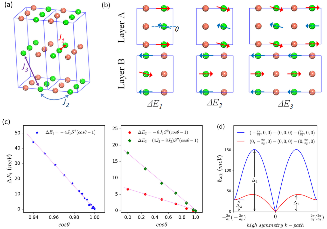
FIG. 4. (a) The primary nearest-neighbor (NN) exchange in Eq. (3). (b) Spin rotation for extraction of J_{1,2,3} . (c) Total energy as a function of the rotation angle. The fitted lines are also shown. (d) In-plane magnon dispersion.
