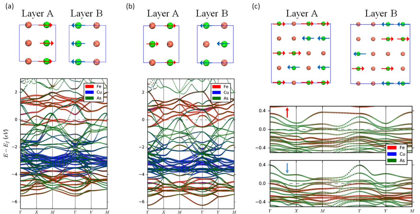
FIG. 2. Three hypothetical atomic and magnetic structures and the corresponding band structures: (a) FM spin configuration, (b) Fe and Cu ions form a checkerboard pattern, and (c) Fe and Cu ions are assumed to distribute randomly. In all these cases, the charge-transfer gap is closed.
