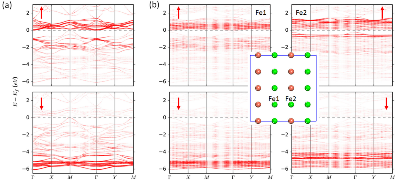
FIG. 3. The effect of interchain Fe as shown by the band structure of (a) \text{NaFe}_{0.5}\text{Cu}_{0.5}\text{As} and (b) \text{NaFe}_{0.53}\text{Cu}_{0.47}\text{As} . The weight of the bands is proportional to the wave-function projection on the Fe site.
