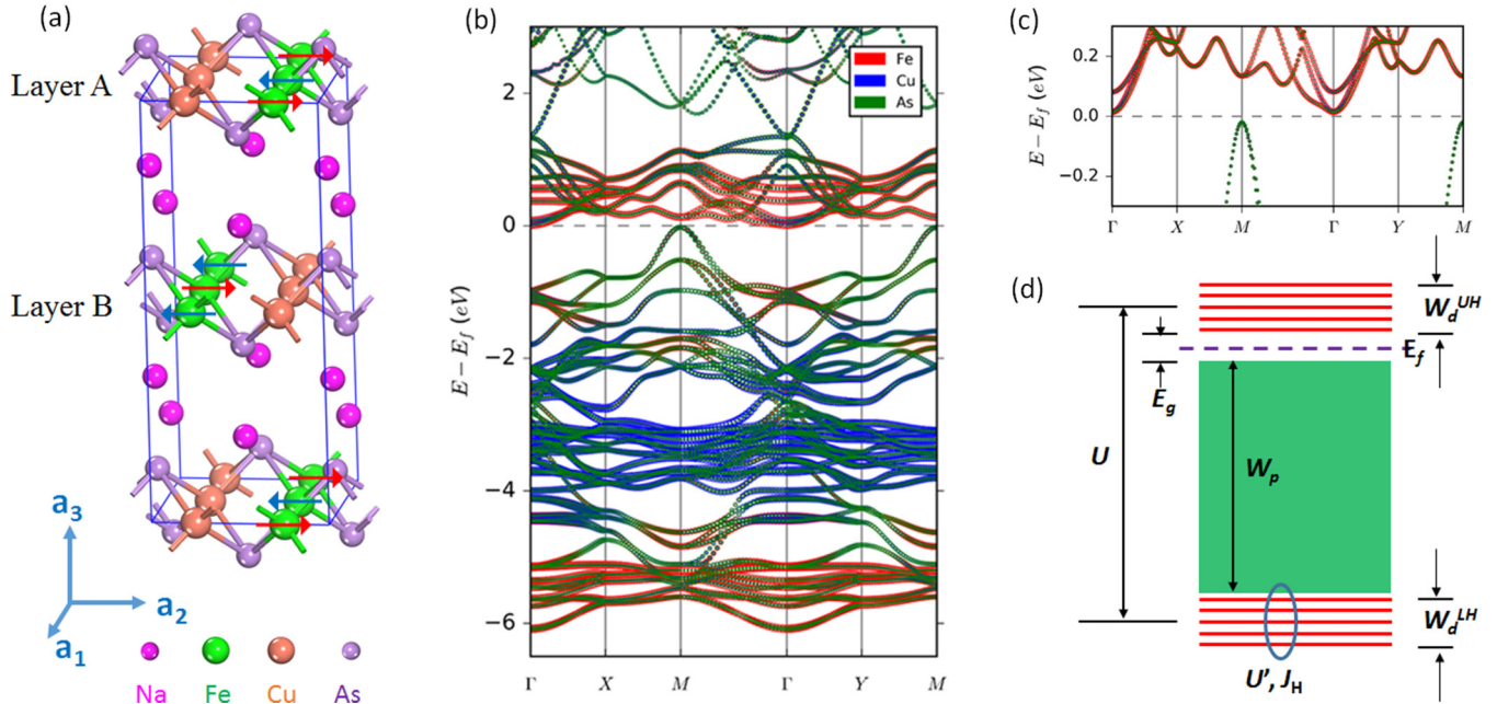
FIG. 1. (a) Crystal and magnetic structure of NaFe 0.5 Cu 0.5 As. Red and blue arrows denote the spin direction. (b) Electronic band structure of NaFe 0.5 Cu 0.5 As, with the atomic composition projection. (c) Zoom-in plot of (b) near the Fermi level. (d) Schematic energy diagram. The key energy scales are summarized in Table I.
