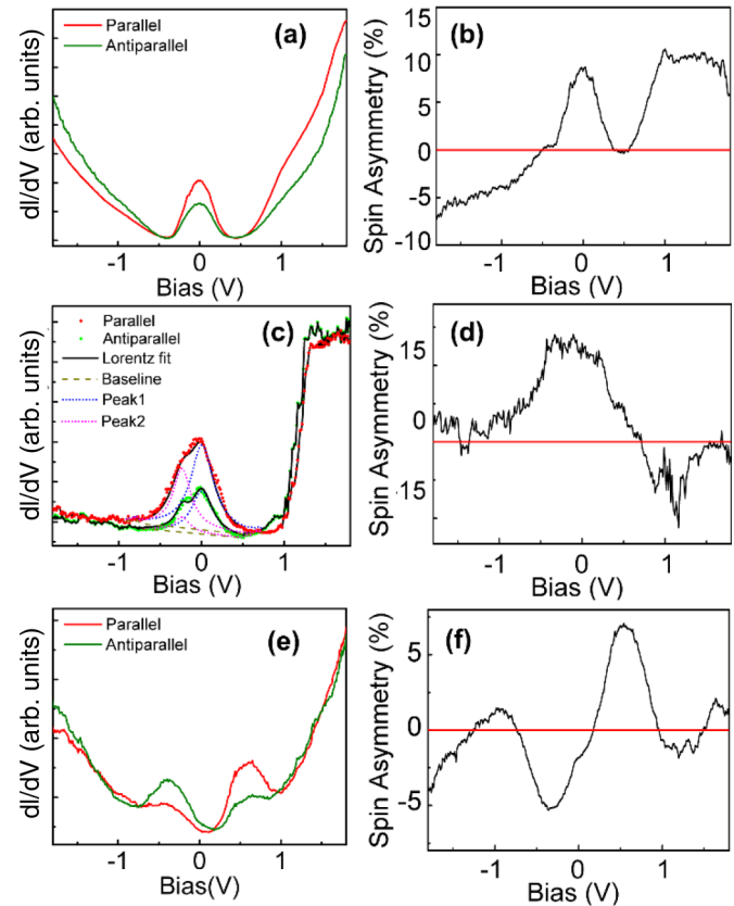
FIG. 2. (a) dI/dV spectra measured for the \text{Cr}(001) surface on parallel (red line) terraces and antiparallel (green line) terraces ( I = 700 \text{ pA} , U = -0.6 \text{ V} ). Each spectrum shown here is an average of 30 point spectra; (c) spin-polarized dI/dV spectra measured on \text{Alq}_3 molecules; and (e) \text{Crq}_3 molecules. Right panels (b), (d), and (f) show the spin asymmetry calculated from the corresponding dI/dV curves to the left.
