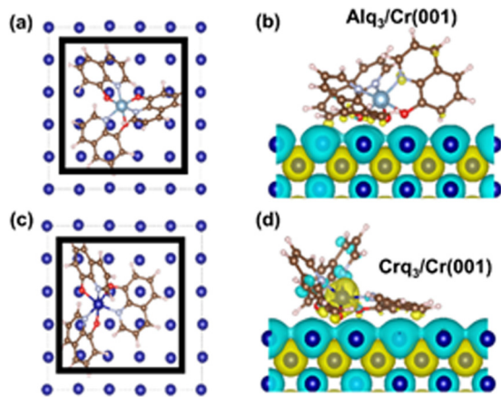
FIG. 3. (a), (c) Top view of the Cr(001) surface upon the adsorption of Alq 3 (a) and Crq 3 (c) molecules, respectively. The dashed squares indicate the unit cell and the solid squares highlight the surface atoms used for PDOS analysis. (b), (d) Side view of Alq 3 (b) and Crq 3 (d) single molecules adsorbed on Cr(001) surface. Both molecules are significantly bent due to interaction with substrate. The blue and yellow colors indicate spin distribution of Crq 3 /Cr(001) and Alq 3 /Cr(001) systems.
