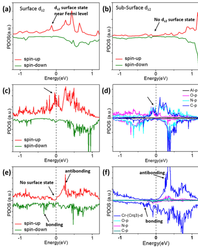
FIG. 4. Projected density of states from DFT calculations. (a) Surface atoms of the Cr(001) substrate with no adsorbates. (b) Bulk atoms in the interior of the Cr(001) slab. (c) Cr surface atoms in the \text{Alq}_3/\text{Cr}(001) system, where a peak remains near the Fermi level (marked by an arrow). (d) An extra peak (marked by an arrow) just below Fermi level is illustrated for the \text{Alq}_3 adsorbate p orbitals on C, O, and N atoms and overlaps the surface state region from (c). (e) In the \text{Crq}_3/\text{Cr}(001) system, the surface state of Cr(001) is not present due to hybridization with the molecule and is replaced by two new peaks separated by a gap labeled as bonding and antibonding. (f) The two new peaks also have significant weight and spin asymmetry in PDOS on the d_z^2 orbital of the \text{Crq}_3 adsorbate.
